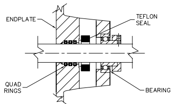
ACST-4 SEAL DETAIL
