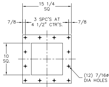
FLANGE DETAIL
