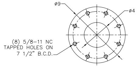
150# FLANGE PATTERN (OPTIONAL)
