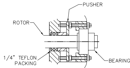
PUSH TYPE SEAL ASSEMBLY
